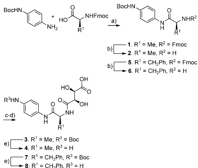
Scheme 4. Synthesis of ylide-aldehyde DNA precursors 4 and 8 .
